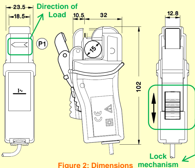
Figure 2: Dimensions
